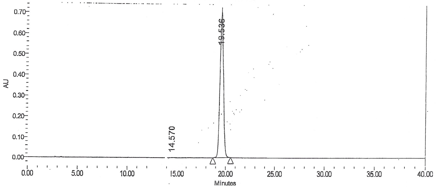
Auto-Scaled Chromatogram
